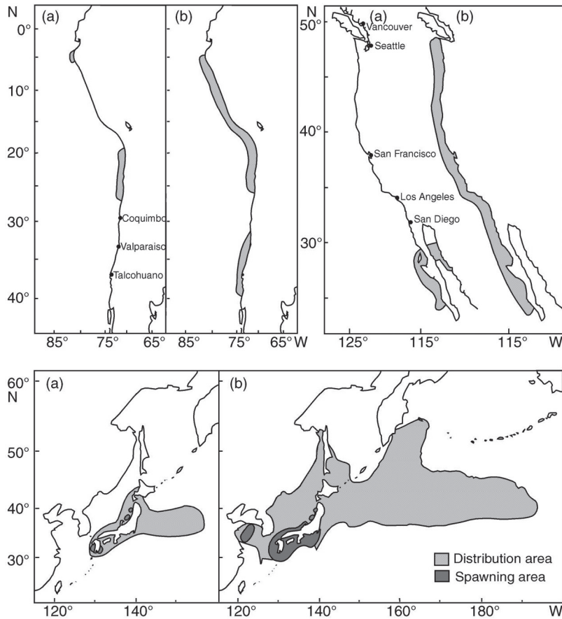
Figure 10. Change in the distribution area of three pelagic fish stocks during (a) low and (b) high abundance periods (Lluch-Belda et al., 1989).
